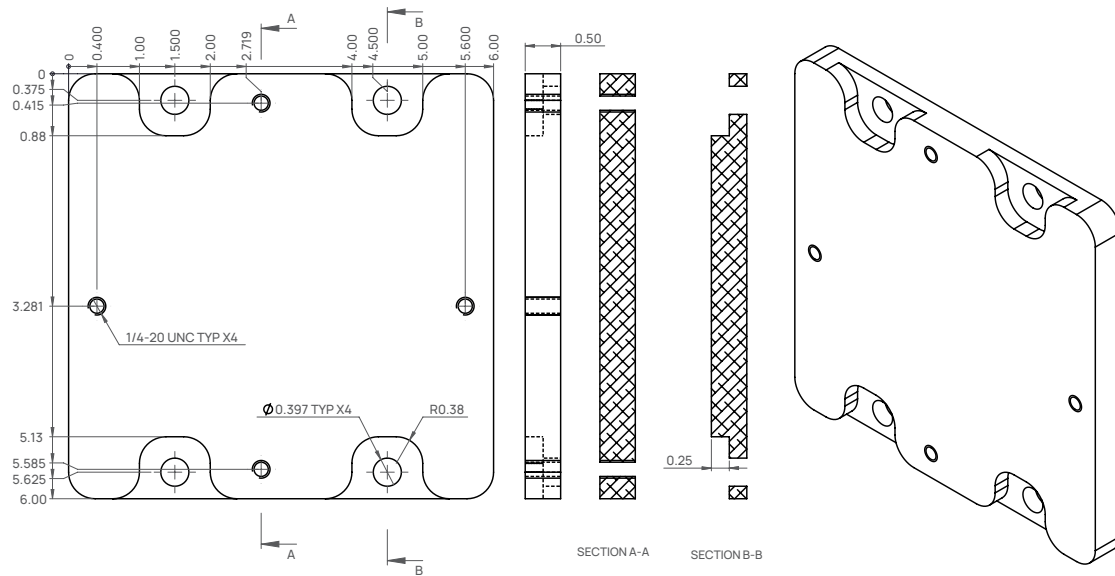
Figure 8 VS2EX to SAVeS Adapter Plate
