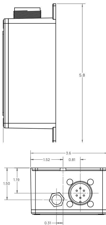
Figure 6 Altronic SAVeS 691816-1C
