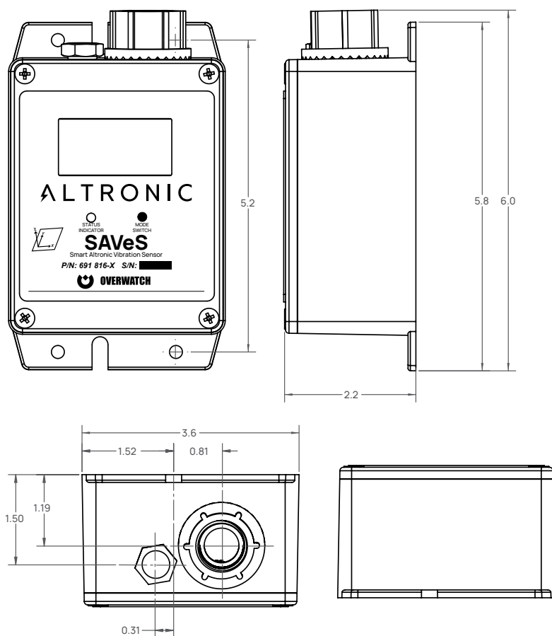
Figure 5 Altronic SAVeS 691816-X
