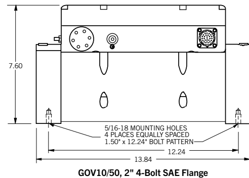
GOV10/50, 2" 4-Bolt SAE Flange
