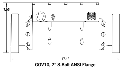
GOV10, 2" 8-Bolt ANSI Flange
