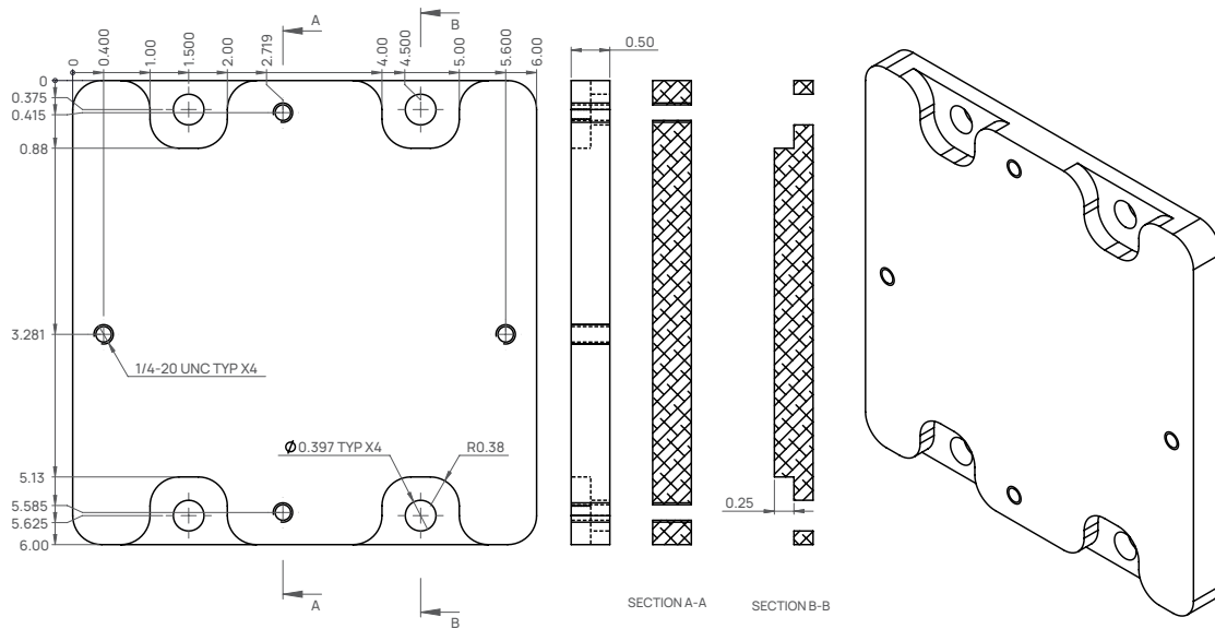
Figure 8 VS2EX to SAVeS Adapter Plate
