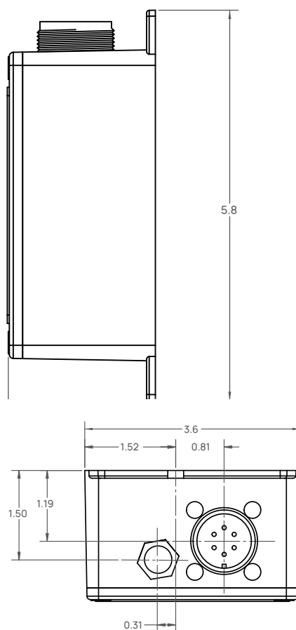
Figure 6 Altronic SAVeS 691816-IC
