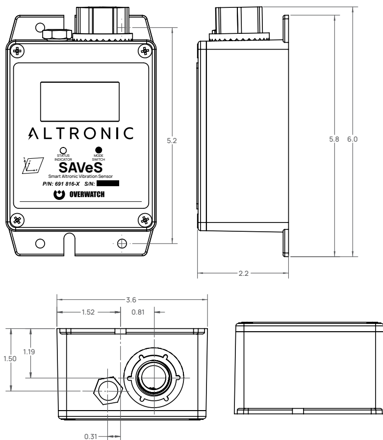
Figure 5 Altronic SAVeS 691816-X
